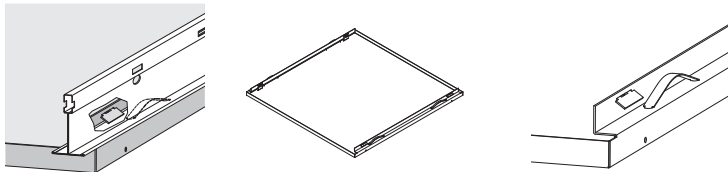
Clip-In Suspension
